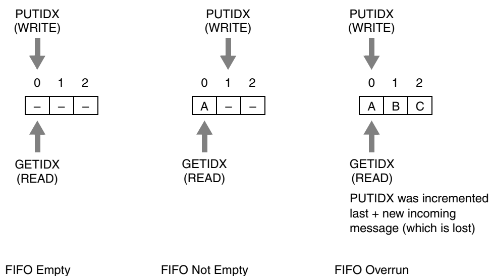
Figure 3-141. FIFO Status (Empty, Not Empty, Overrun) — Example of FIFO with Three Message Buffers
